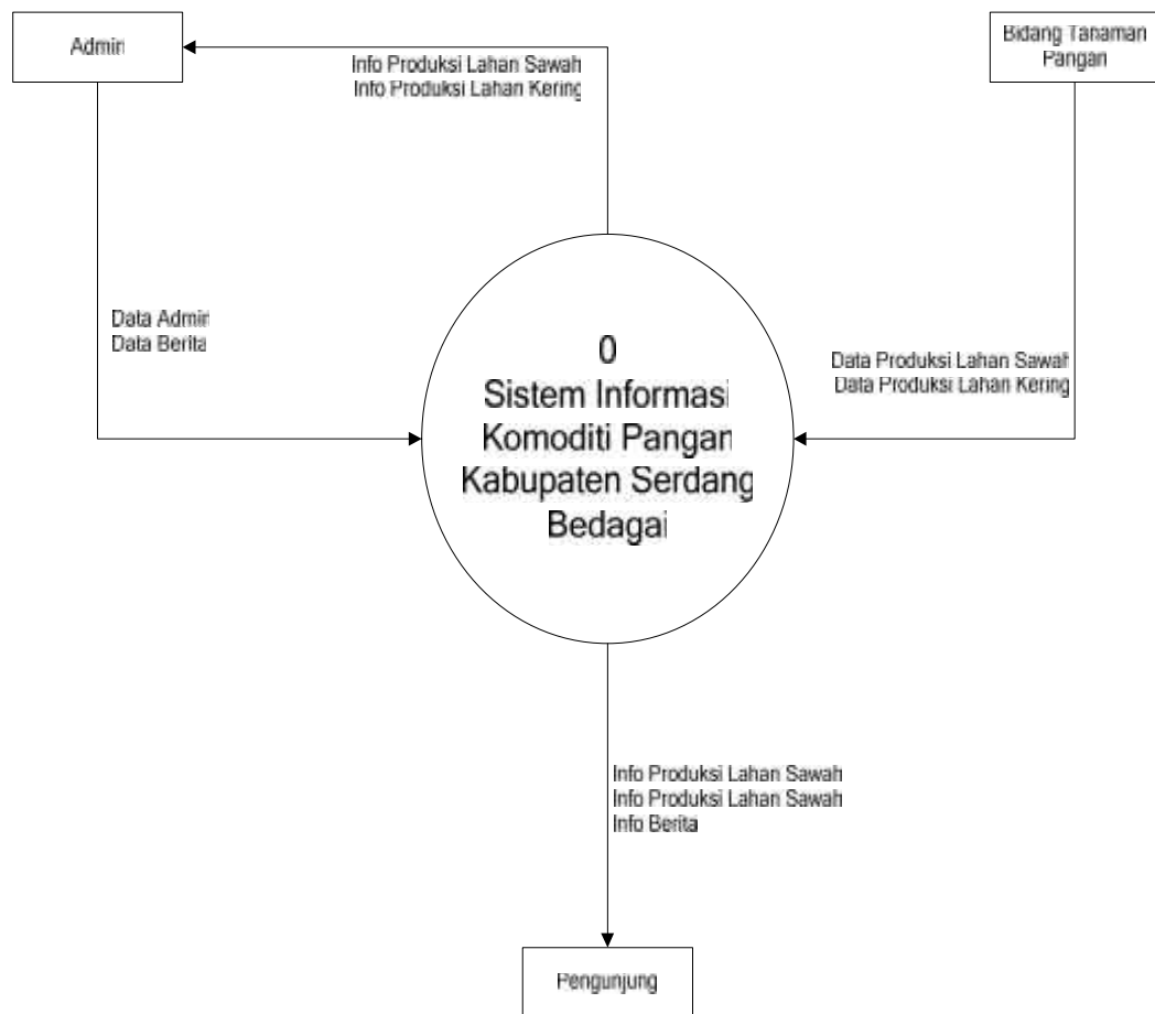
Lampiran 3. Diagram konteks
