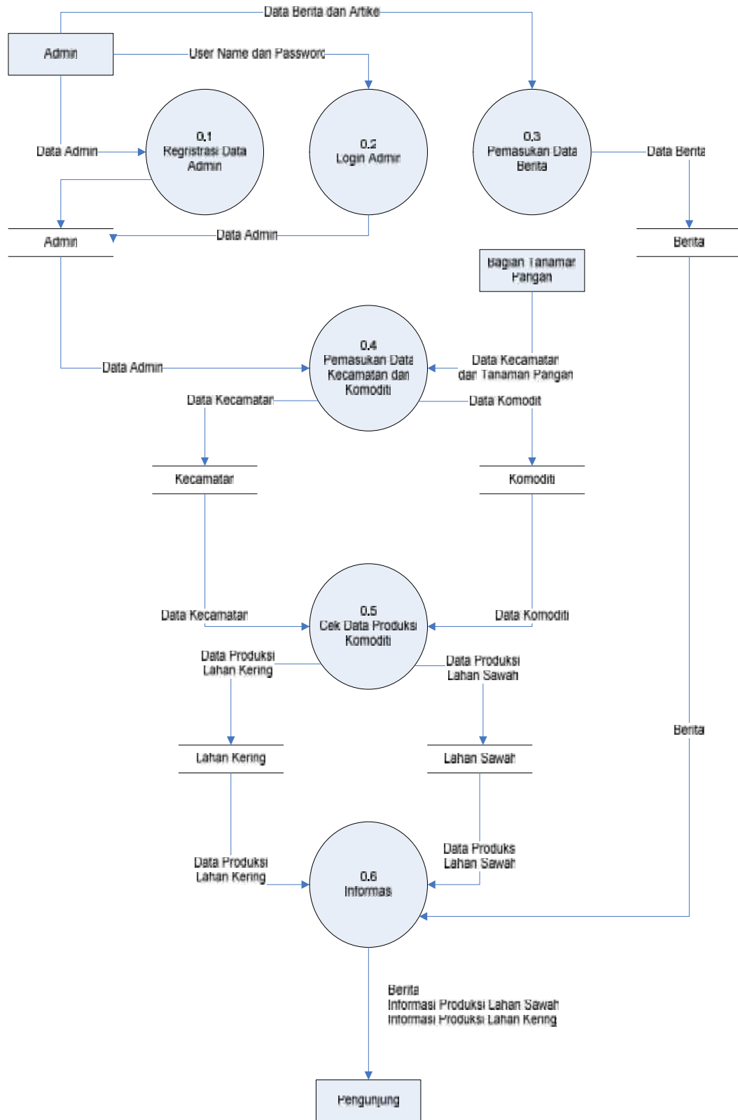
Lampiran 4. Data flow digram (DFD) level nol
